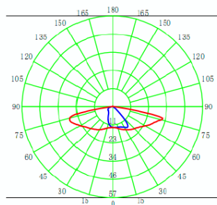
Photometric Light Plot
